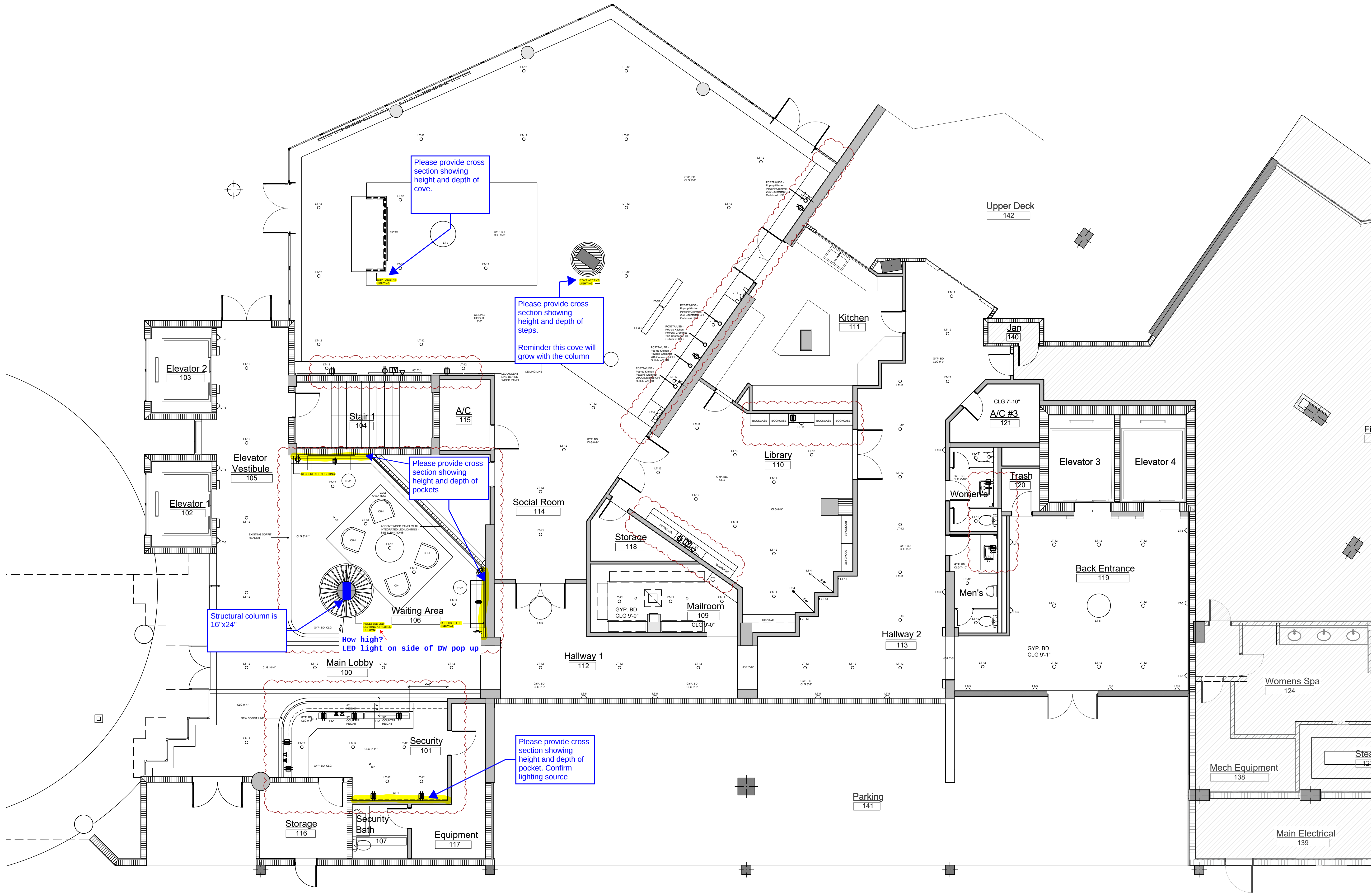
POWER PLAN 3/16"=1'-0"
